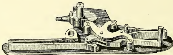
Lock of Murcott's Hammerless Gun.
